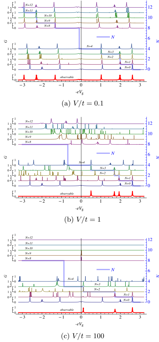
Figure 12.4: Conductance profiles in the case of a flux per plaquette \phi = \pi/2 (created by a uniform magnetic field). All other parameters are the same as in Fig. 12.3. An additional peak corresponding to the transition between 3 and 4 particles is present for small and intermediate V/t , but absent for large V/t .
