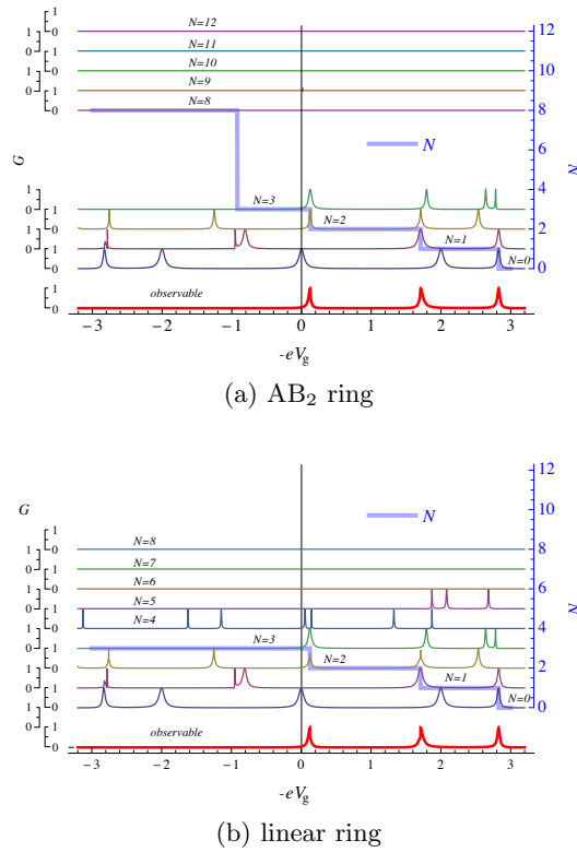
Figure 12.5: Conductance profile as a function of the gate voltage for: (a) an AB_2 ring with N_c = 4, V = 100, \omega = 0 and t_L = t_R = 0.3t with contacts at opposite sites A; (b) the equivalent linear ring, with the same parameters but ring hoppings renormalized as t \rightarrow \sqrt{2}t and leads contacts at opposite sites.
